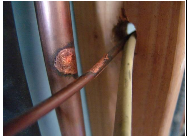
Figure 6: Horizontal ground wire discharge to vertical copper pipe.
