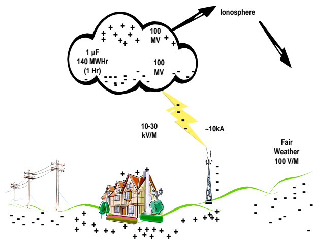
Figure 1: Lightning discharge
