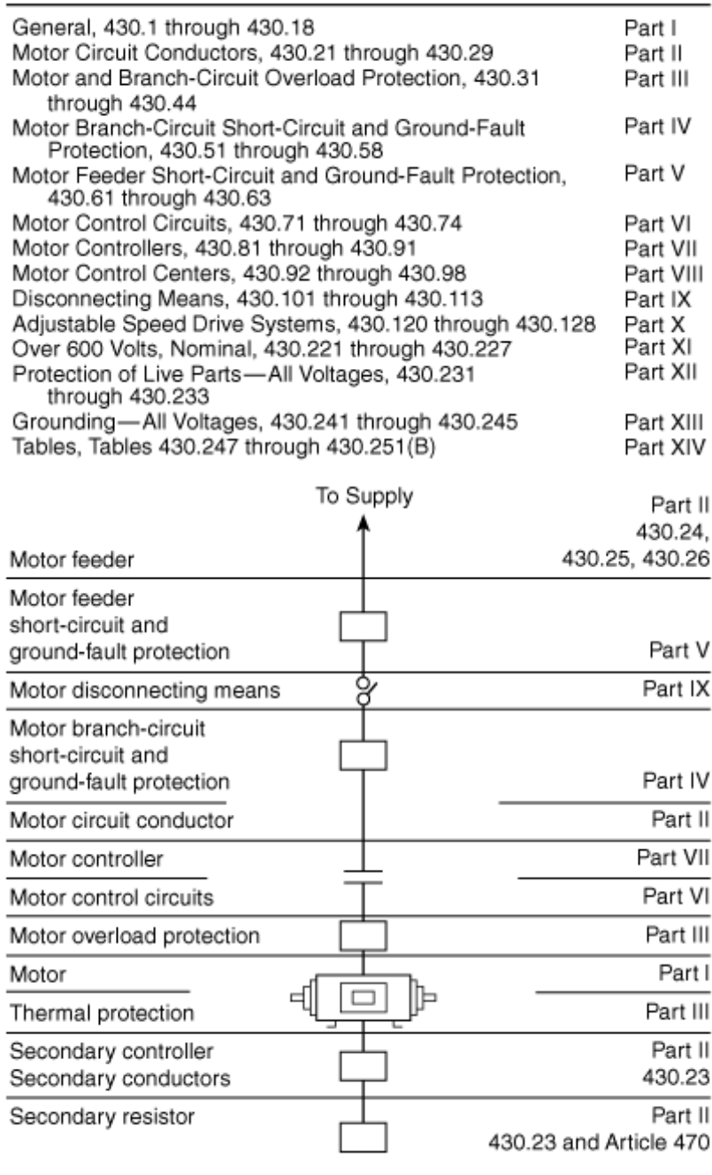
Figure 430.1 Article 430 Contents
