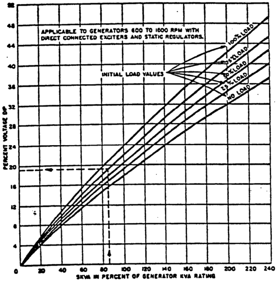
Figure 3: Voltage Dip with Motor Starting Loads
