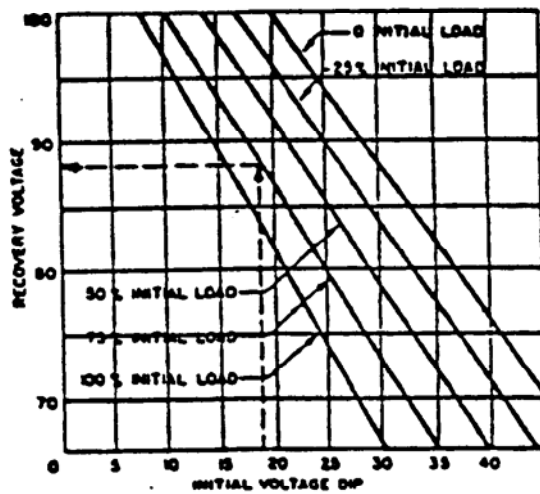
Figure 4: Recovery Voltage for Generators with Static Regulators and High Speed Excitation
